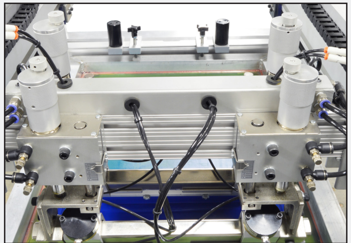
Solid chopper assembly on up-graded units provides consistent, even ink deposit and reduces deflection.
